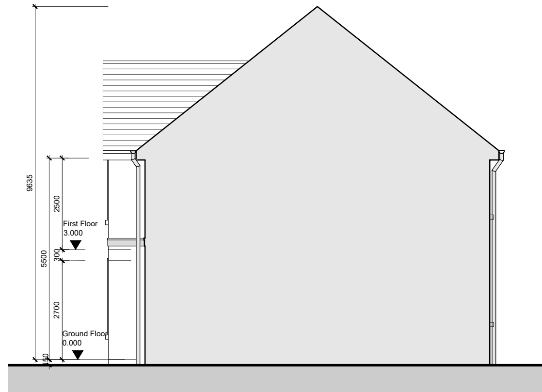
Side Elevation 02
