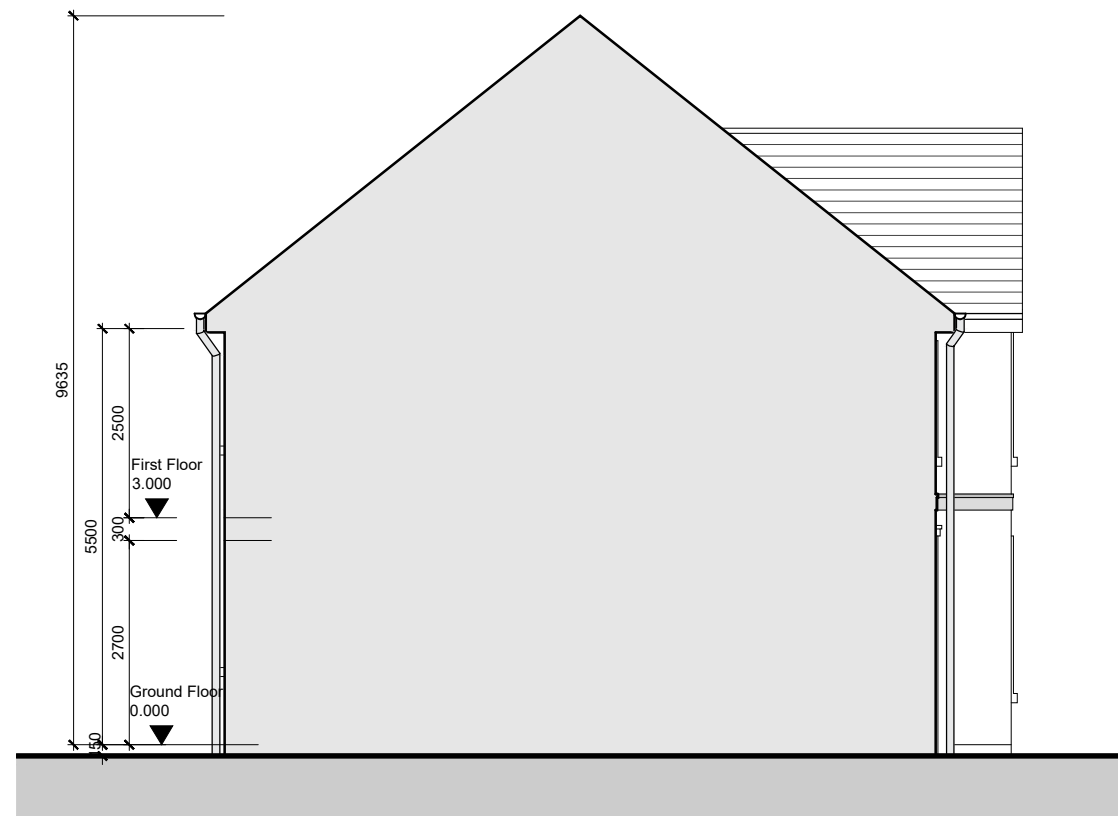
Side Elevation 01
